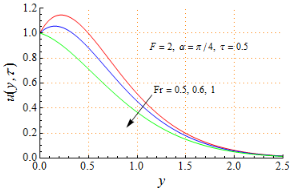
Fig. 1. Velocity profile on varying F_r (small)
