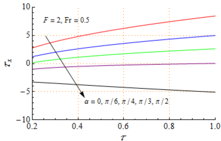
Fig. 7. Variation of shear stress on varying \alpha and time \tau
