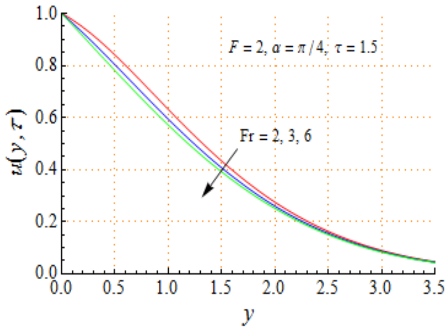
Fig. 2. Velocity profile on varying F_r (large)
