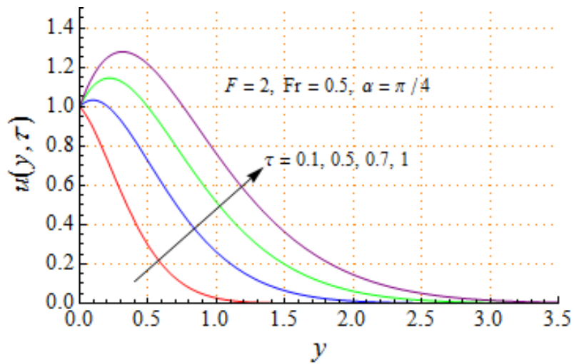
Fig. 5. Velocity profile on varying time \tau
