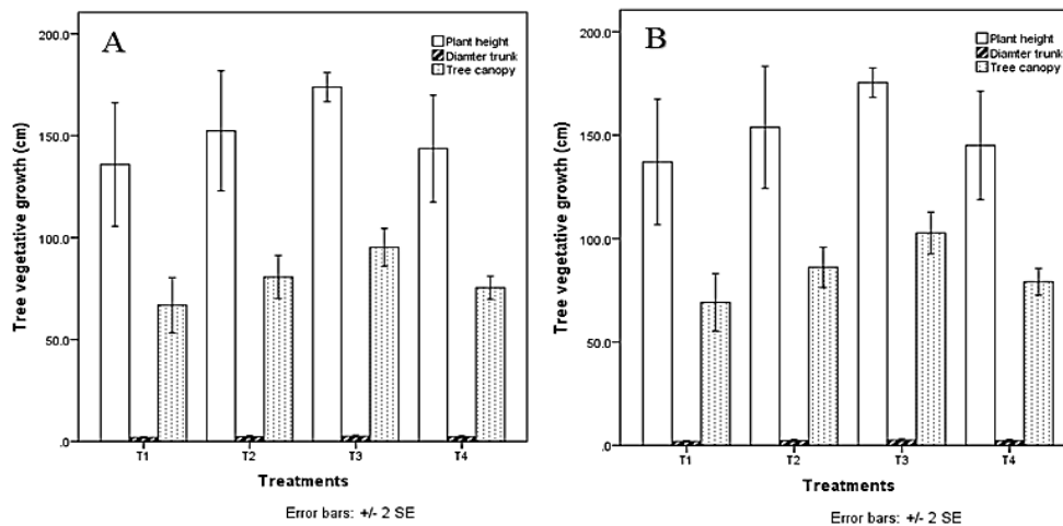
Fig. 1. Effect of micro-organic fertilizer on plant height, diameter trunk and tree canopy of M.suavis species (A: spring season 2023; B: summer season 2023)
