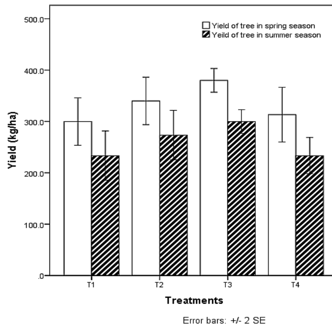
Fig. 2. Effect of micro-organic fertilizer on yield of M.suavis species
